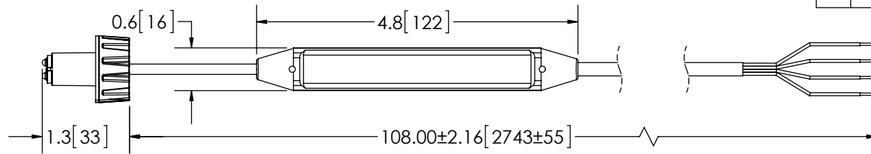
RIGHT VIEW
